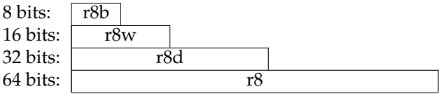
Figure 10.2: X86 Register Structure
